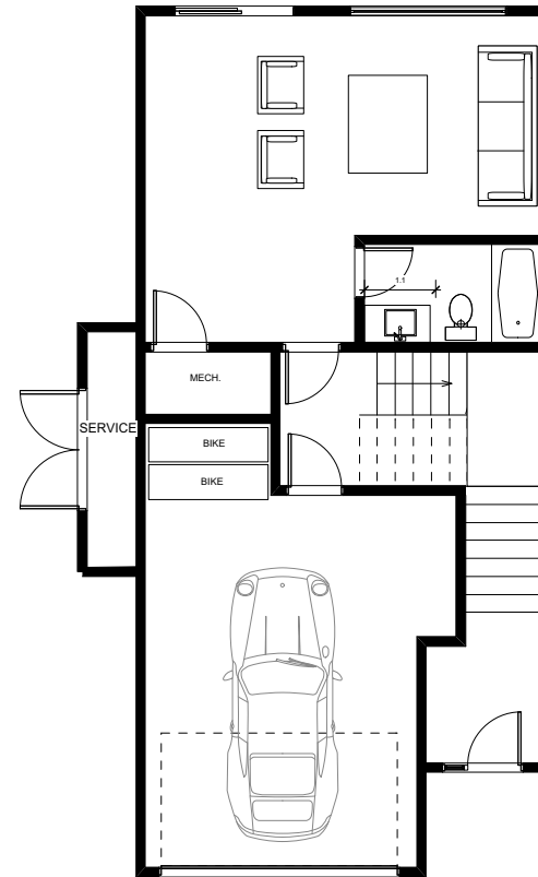
LOWER LEVEL FLOOR PLAN - 533 sq ft
